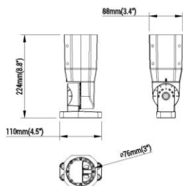
Ø76mm Slipfitter
