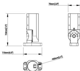
Ø60mm Slipfitter
